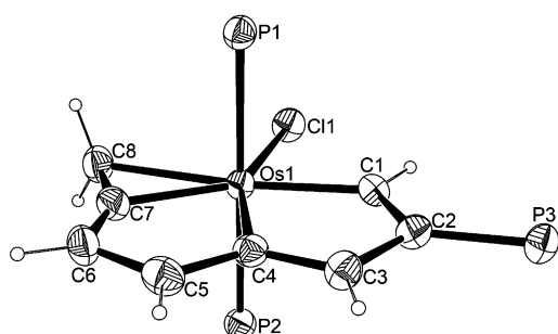
Figure 1. Molecular structure of the cation of 2 (drawn with 50% probability). The phenyl moieties in \text{PPh}_3 have been omitted for clarity. Selected bond lengths [Å] and angles [deg]: Os1–C1 2.021(5), Os1–C4 2.076(5), Os1–C7 1.996(5), Os1–C8 2.272(5), C1–C2 1.401(8), C2–C3 1.412(8), C3–C4 1.381(8), C4–C5 1.414(8), C5–C6 1.378(8), C6–C7 1.387(8), C7–C8 1.376(8); Os1–C1–C2 120.0(4), C1–C2–C3 113.0(5), C2–C3–C4 113.0(5), C3–C4–Os1 118.7(4), C4–Os1–C1 75.2(2), Os1–C4–C5 119.3(4), C4–C5–C6 112.5(5), C5–C6–C7 111.0(5), C6–C7–Os1 124.4(4), C7–Os1–C4 72.8(2), Os1–C7–C8 82.5(4), C7–C8–Os1 60.6(3), C8–Os1–C7 36.9(2).
