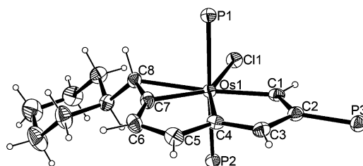
Figure 2. Molecular structure of the cation of 3 (drawn with 50% probability). The phenyl moieties in \text{PPh}_3 have been omitted for clarity. Selected bond lengths [Å] and angles [deg]: Os1–C1 2.040(4), Os1–C4 2.080(4), Os1–C7 1.997(4), Os1–C8 2.368(4), C1–C2 1.381(6), C2–C3 1.414(6), C3–C4 1.392(6), C4–C5 1.407(6), C5–C6 1.371(7), C6–C7 1.375(7), C7–C8 1.396(6); Os1–C1–C2 120.0(3), C1–C2–C3 113.6(4), C2–C3–C4 112.8(4), C3–C4–Os1 118.6(3), C4–Os1–C1 74.94(17), Os1–C4–C5 119.5(3), C4–C5–C6 112.7(4), C5–C6–C7 110.3(4), C6–C7–Os1 125.4(3), C7–Os1–C4 71.79(18), Os1–C7–C8 86.6(3), C7–C8–Os1 57.3(2), C8–Os1–C7 36.06(17).
