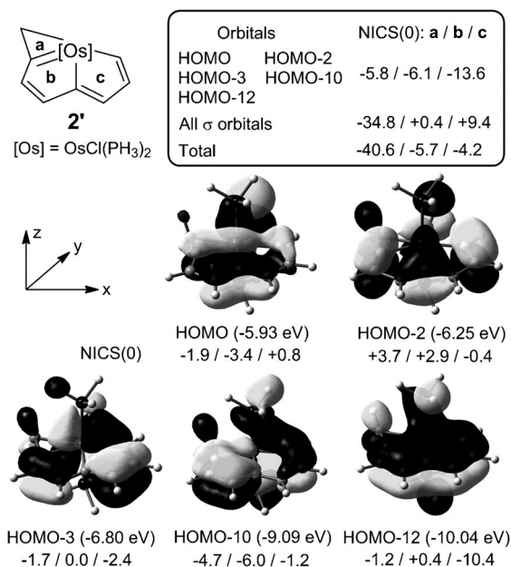
Figure 3. Key occupied \pi MOs and their energies together with their contributions to NICS(0) (in ppm) for the model complex 2' . The eigenvalues of the MOs are given within parentheses in the first line whereas the NICS(0) values of rings a, b, and c are given in the second line.
